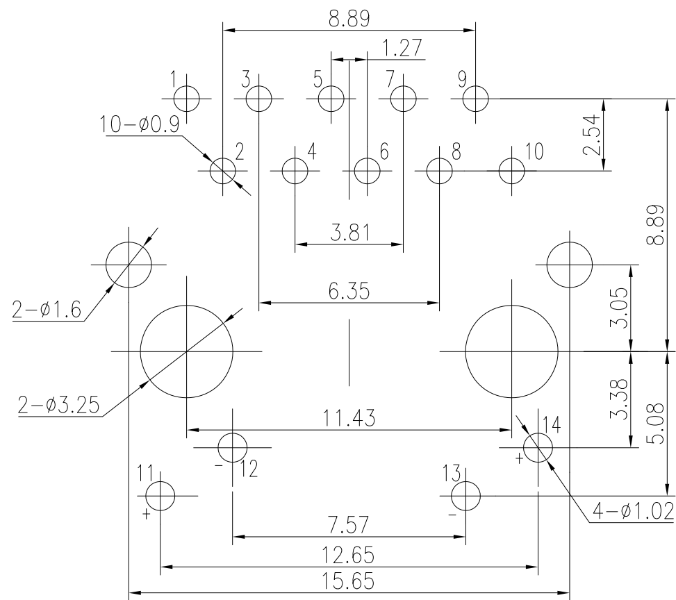
SUGGESTED PCB LAYOUT (TOP VIEW) DIMENSIONAL TOLERANCE: .XX ±0.05[0.002]
