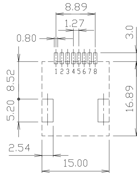
PCB LAYOUT Ref.
