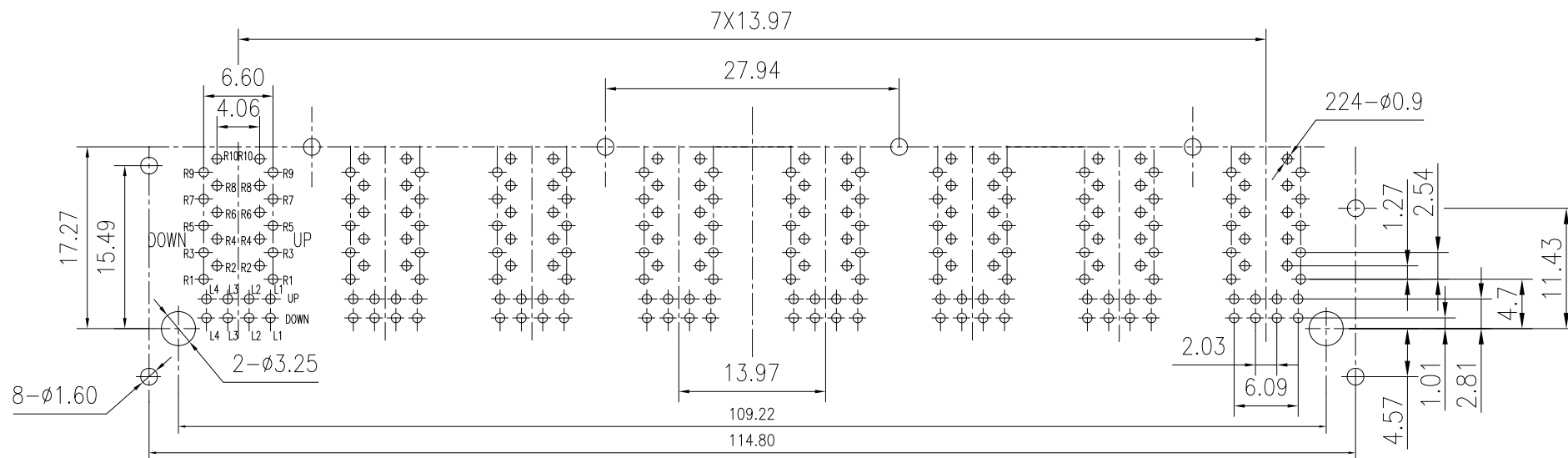
SUGGESTED PCB LAYOUT
