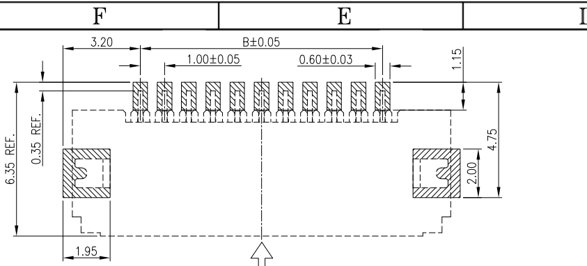
FFC/FPC INSERT DIRECTION RECOMMEND PCB LAYOUT 04~30PIN Situation
