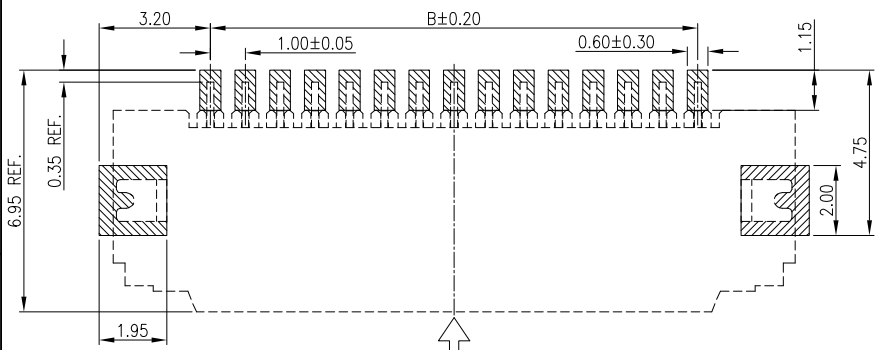
FFC/FPC INSERT DIRECTION RECOMMEND PCB LAYOUT 31~60PIN Situation
