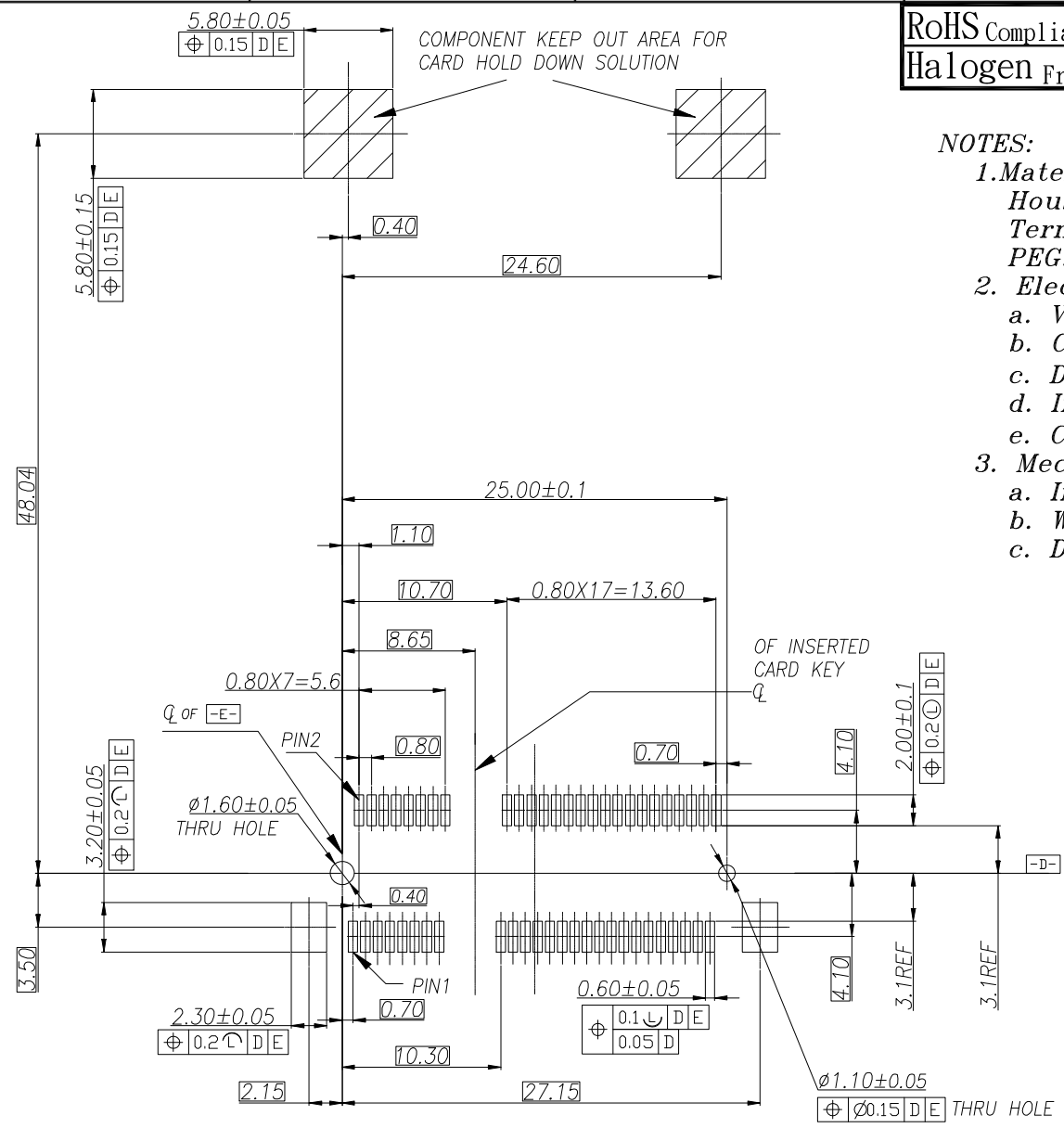
RECOMMENDED PCB LAYOUT THICKNESS: 1.20±0.05mm
