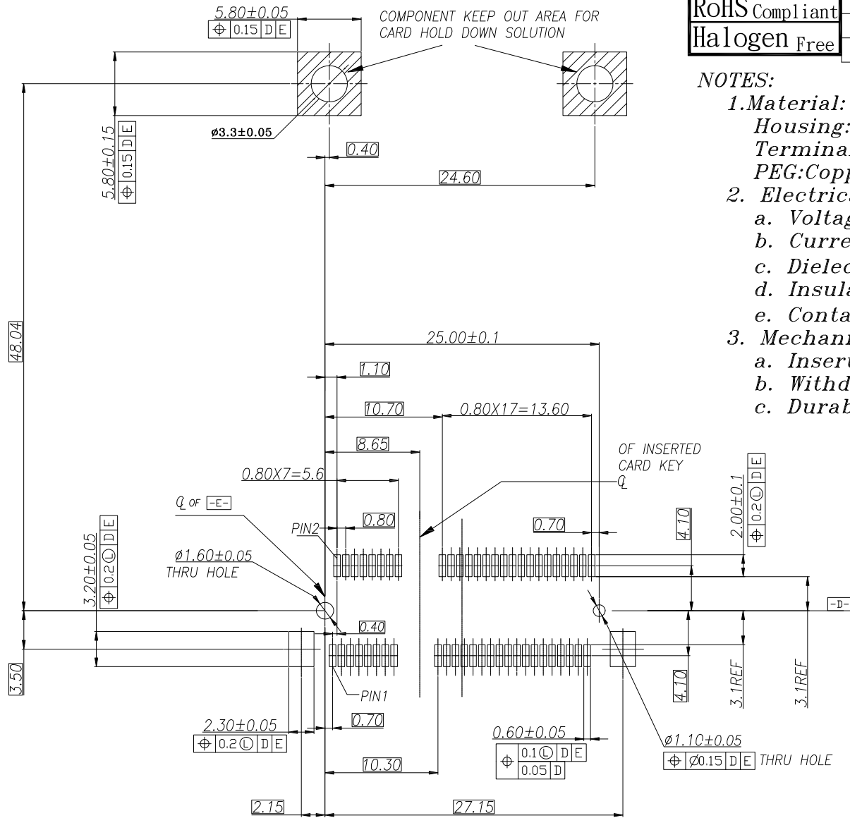
RECOMMENDED PCB LAYOUT THICKNESS: 1.20±0.05mm
