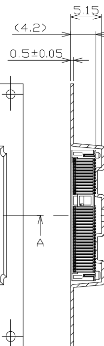
SECT B-B
