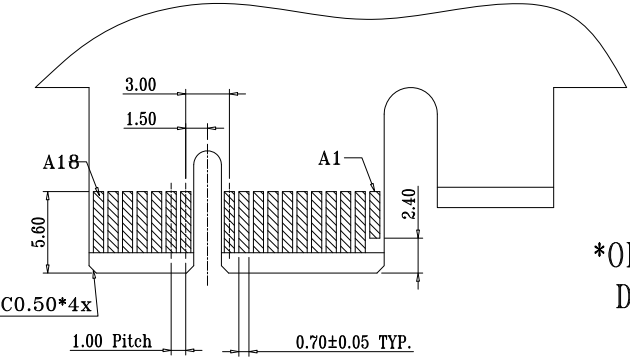
RECOMMENDED EDGE CARD PATTERN(SECONDARY SIDE)
