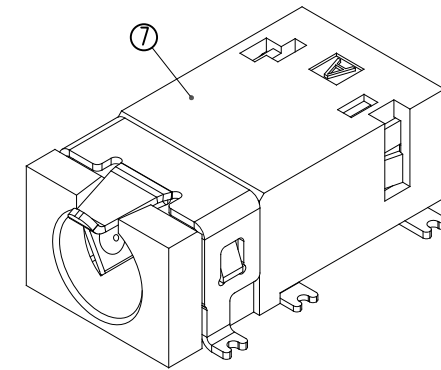
NOTES: 1. CONTACT CURRENT RATING: 12V/1A. 2. CONTACT RESISTANCE: 50 mΩ MAX.; 3. INSULATION RESISTANCE: 100MΩ MIN.; 4. DIELECTRIC WITHSTANDING: 500V AC MIN.; 5. DURABILITY: 5,000 CYCLES MIN.; 6. CONNECTOR MATING FORCES: 29.4N (3.00Kgf) MAX.; 7. CONNECTOR UNMATING FORCES: 2.94N(0.30Kgf) MIN. 8. THE PRODUCT MACHINE WITH A GAP THAT: THE FINISHED MACHINE WITH SOCKET BEFORE/ UP/DOWN/LEFT/RIGHT SIDE OF 8, PROTECTION GAP FIRST PROPOSED THE DESIGN OF 0.15mm.
