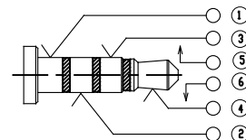
AFTER INSERT SCHEMATIC
